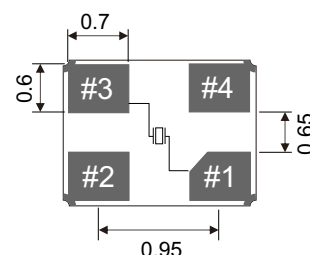
Pad Pattern
