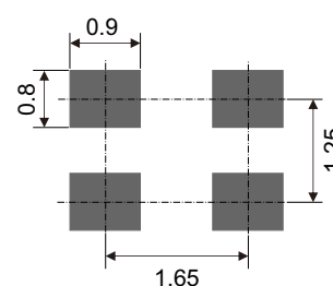
Pad Pattern
