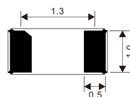
Pad Pattern
