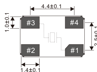
Pad Pattern
