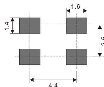
Pad Pattern
