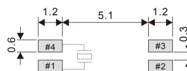
Pad Pattern
